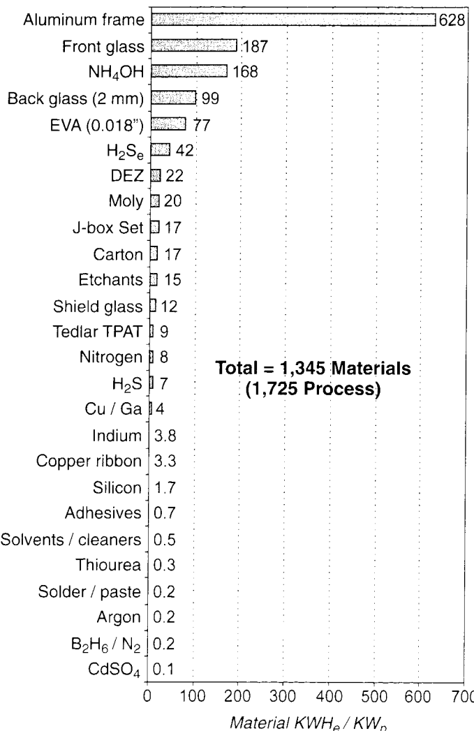
Figure 3b: Materials Energy Content: ST40
