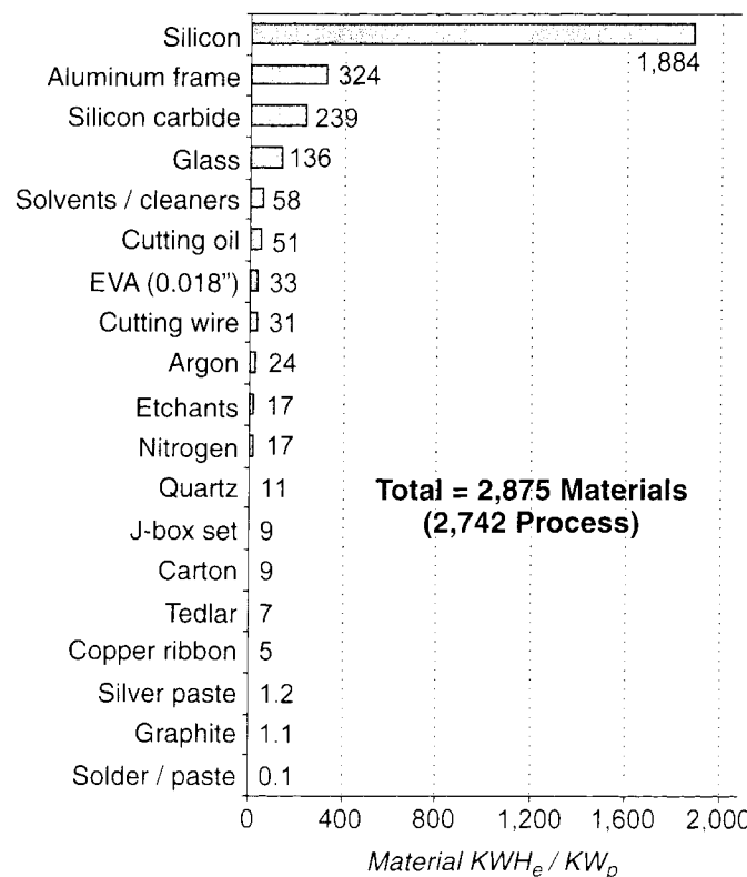
Figure 3a: Materials Energy Content: SP75
