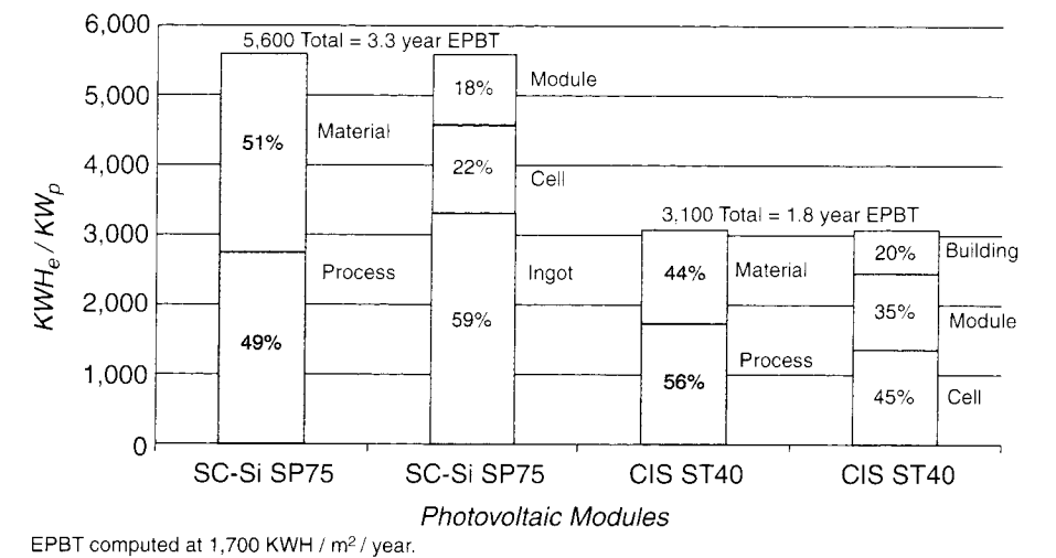
Figure 4: Energy Requirements Breakdown
